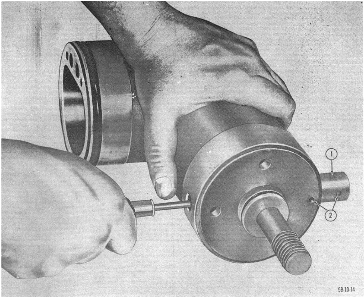
Figure 14. Pushing out venturi assembly from its cavity (Model 4310CA).
