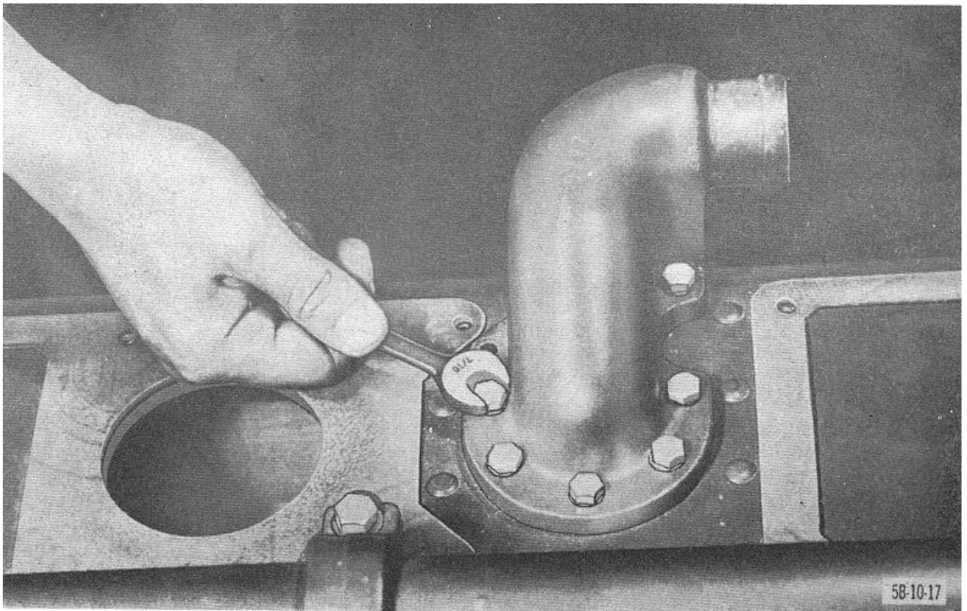
Figure 17. Removing T-mounting.
